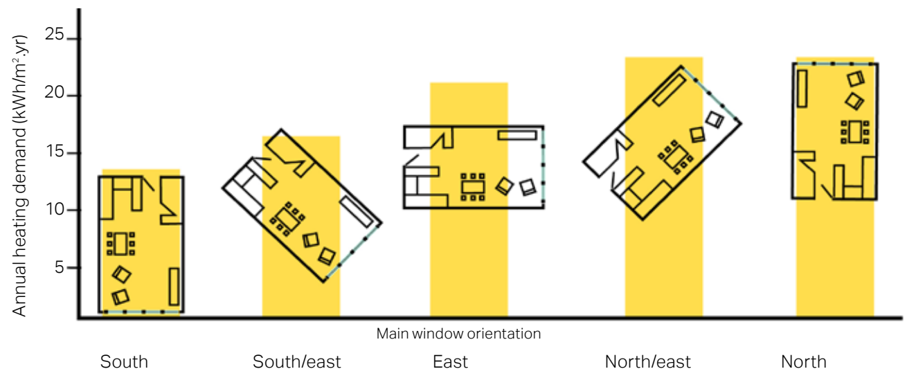
Figure 70: An illustrative graph showing solar orientation of a room against the annual heating demand.
