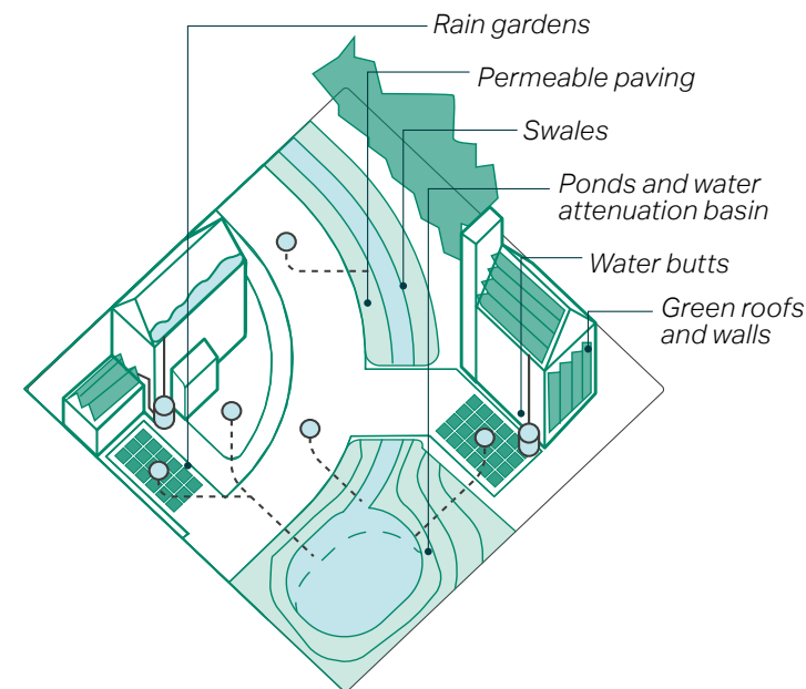
Figure 74: Diagram showing the best use of harvesting water systems, rain garden, swales, permeable paving and green roofs.
