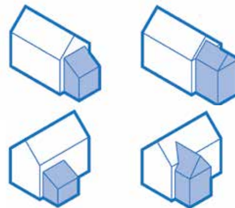
Figure 57: Examples for incorporating side extensions that considers the mass, scale, orientation and building line of the original building.
